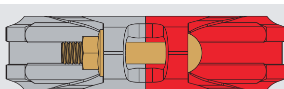
The straight seat design of the PicoFix Type 901 pipe coupling compensates for inaccuracies.
