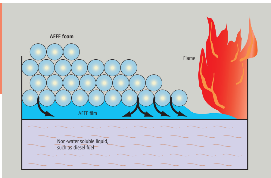
Principle drawing: Water film development (AFFF effect)
